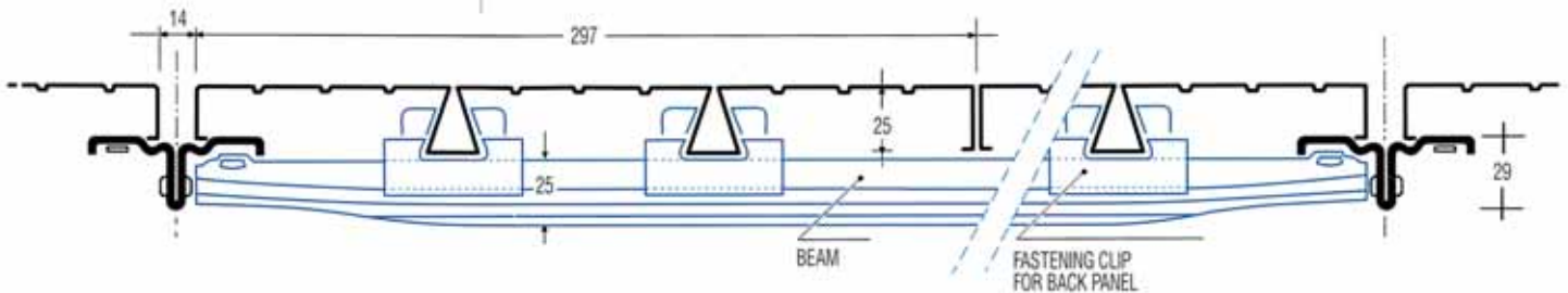
BACK PANEL H 12 FOR BACK-TO-BACK BAYS
